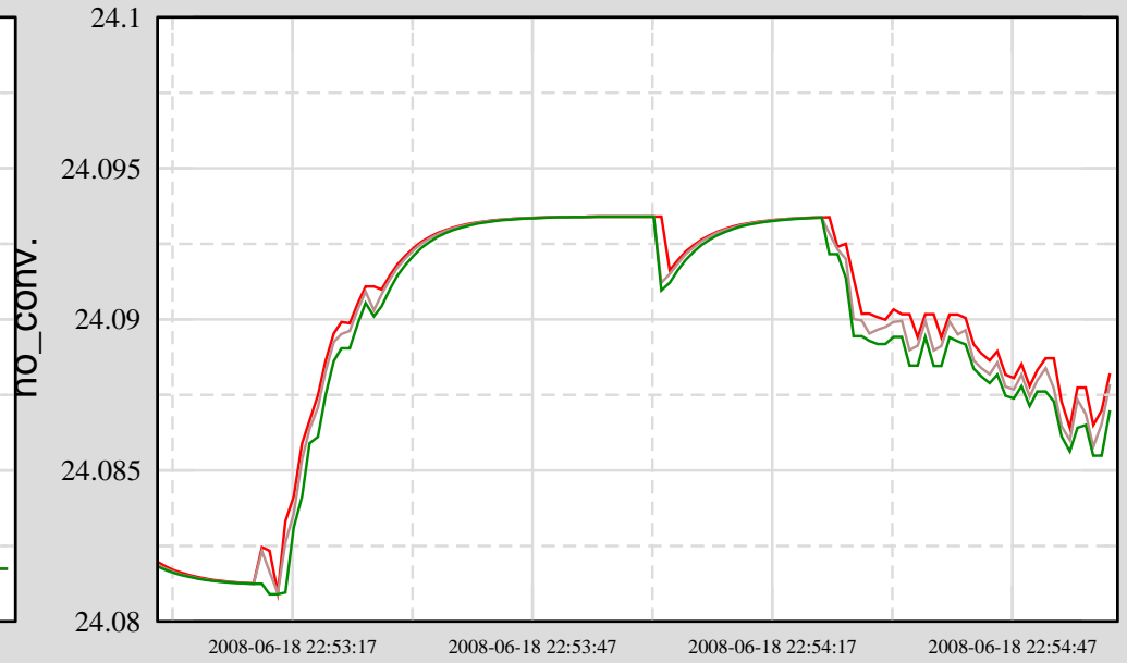
Ch 11: C1:PSL-126MOPA_DTMP
