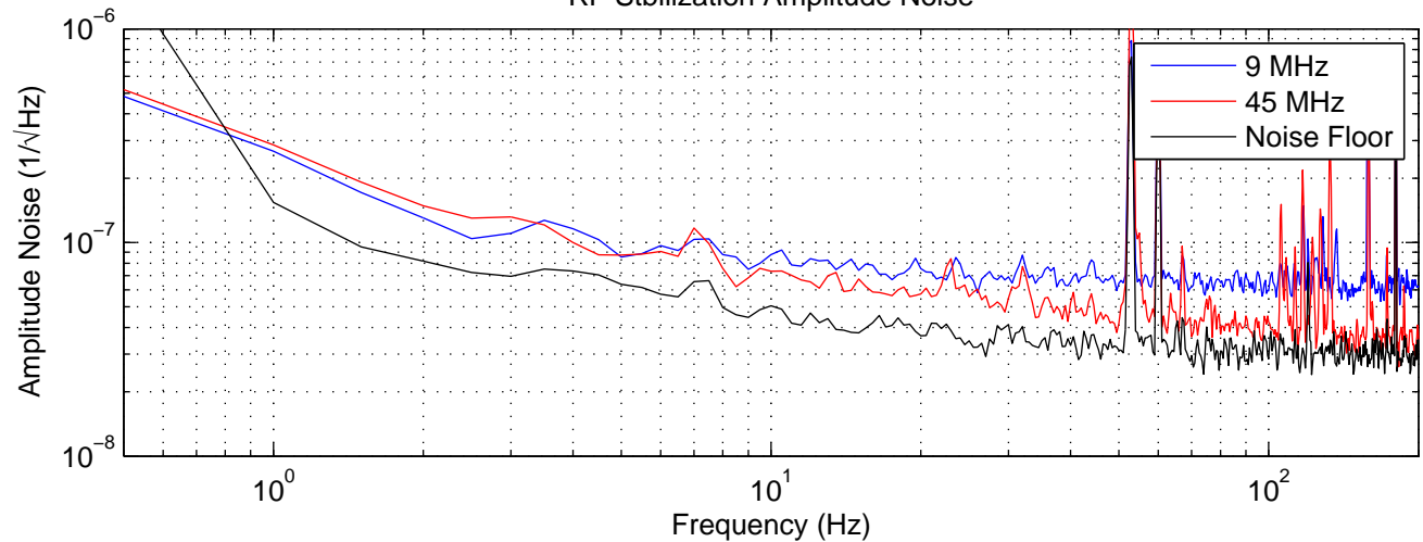
RF Stabilization Amplitude Noise
