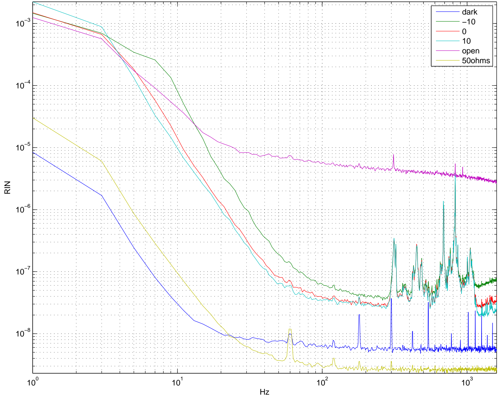
ISS RIN seen by monitor photodiode
