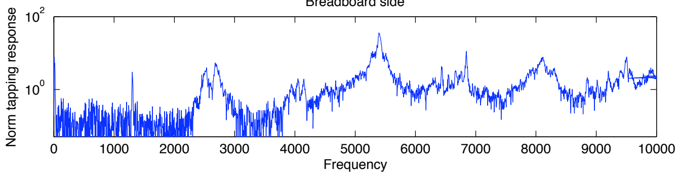
Breadboard side
